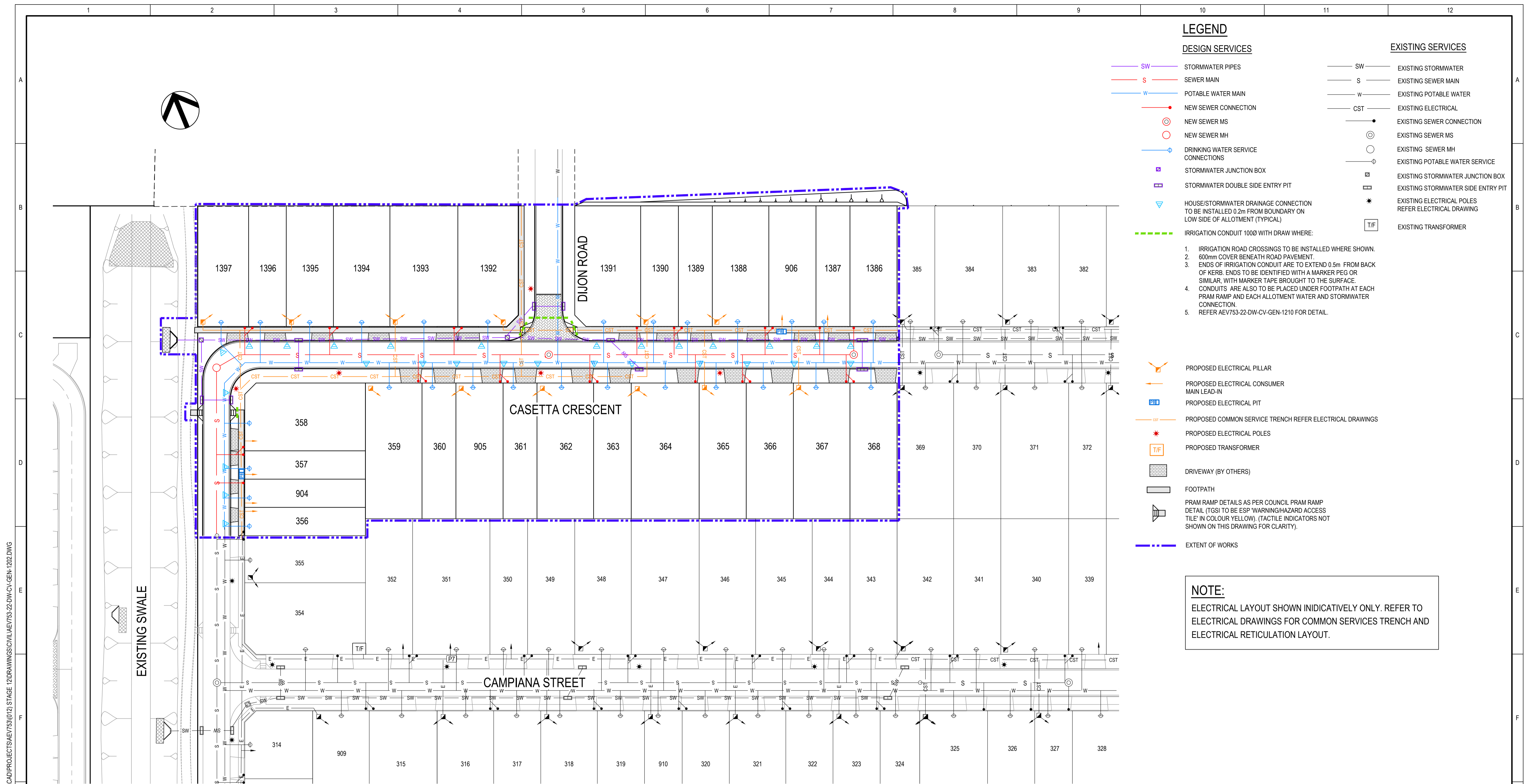
SERVICE LAYOUT PLAN SCALE 1: 500
