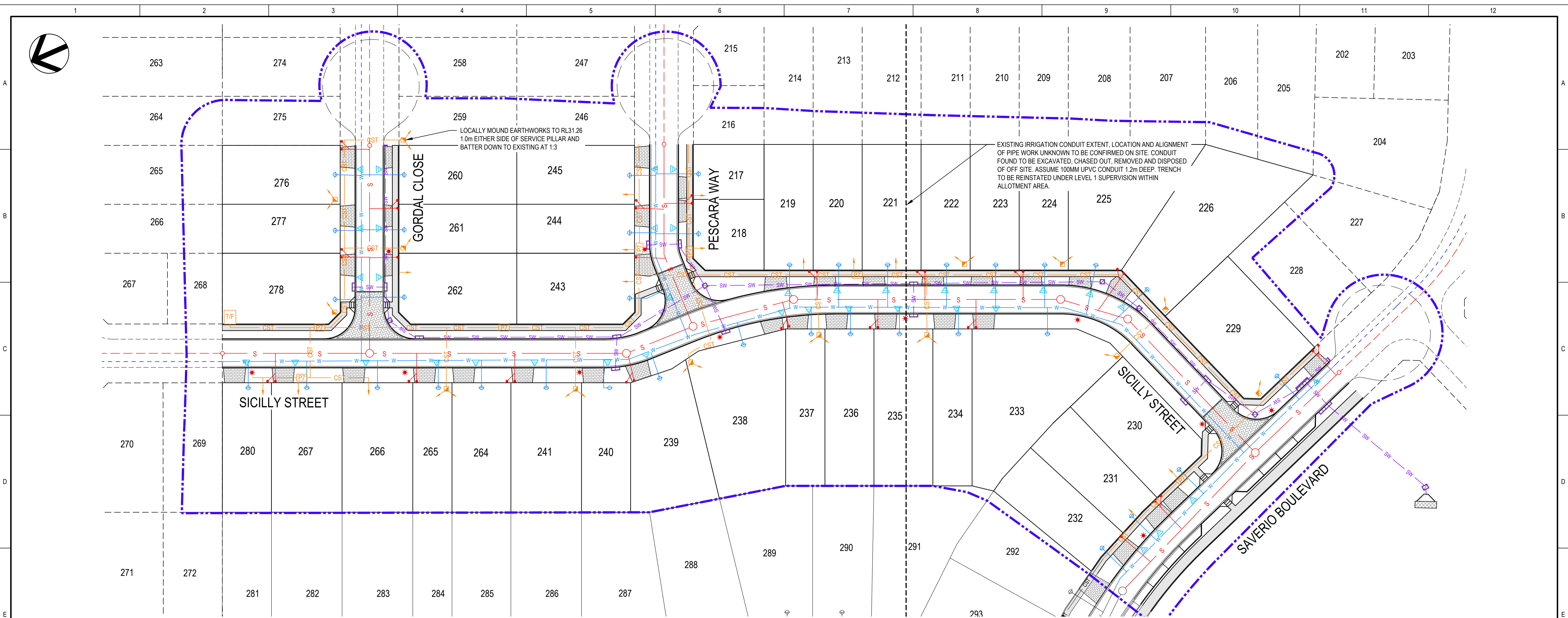
SERVICE LAYOUT PLAN SCALE 1: 500
